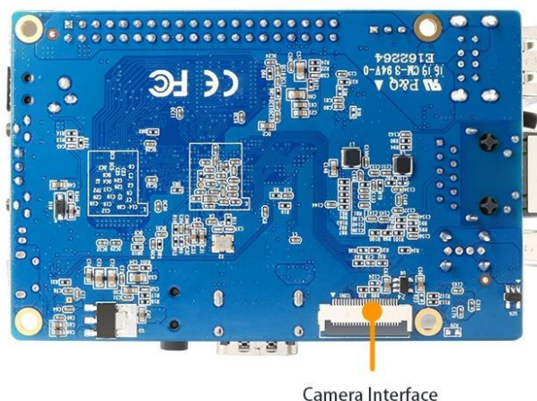
Camera Interface
